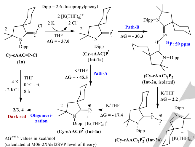
Scheme 4. Mechanism for the generation of cAAC-supported potassium-phosphinidenides 2a/3-4 in THF (see SI for Me _2 -cAAC analogs).
