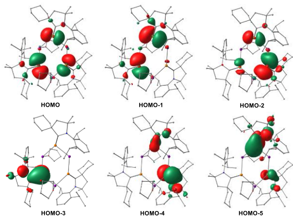
Figure 6. Representative Molecular Orbitals of complex 5 at M06-2X/def2TZVPP level of theory. Hydrogen atoms are omitted for clarity.
