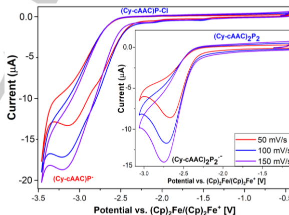
Figure 1. Cyclic voltammograms of \text{Cy-cAAC=P-Cl} ( 1a ) (left) and (\text{Cy-cAAC})_2\text{P}_2 ( Int-2a ) (inset) in THF containing 0.1 M [n\text{-Bu}_4\text{N}]\text{PF}_6 as the electrolyte (CE: Pt, WE: GC, RE: Ag).
