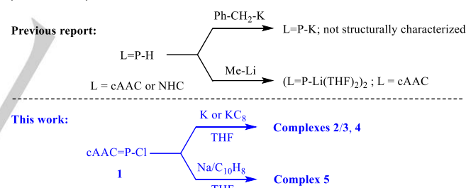
Scheme 1. Synthetic routes for metal-phosphinidenes.
