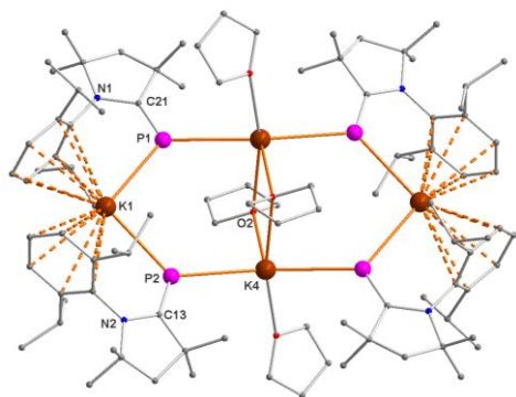
Figure 4. Molecular structure of complex 4·2THF . Hydrogen atoms and two solvated THF molecules were omitted for clarity. Important bond lengths [Å] and bond angles [°]: C21-P1 1.702(3), C13-P2 1.703(3), C21-N1 1.402(3), C13-N2 1.401(3), P1-K1 3.2893(10), P2-K1 3.2314(9), P1-K4 3.2761(10), P2-K4 3.3532(10), K4-O1 2.885(3), K4-O2 2.763(3) and 2.954(3), N1-C21-P1 126.53(19), N2-C13-P2 127.93(19), C21-P1-K4 120.86(9), C21-P1-K1 115.19(9), K1-P1-K4 123.87(3), P2-K1-P1 97.49(2).
