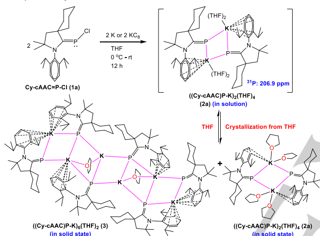
Scheme 2. Synthesis of cAAC-supported dimeric [((\text{Cy-cAAC})\text{P-K})_2(\text{THF})_4] ( 2a ) and hexameric [((\text{Cy-cAAC})\text{P-K})_6(\text{THF})_2] ( 3 ) potassium-phosphinidenes.
