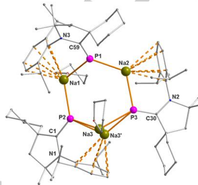
Figure 5. Molecular structure of complex 5·2THF . Hydrogen atoms and two solvated THF molecule were omitted for clarity. Both coordinated THF molecules have half occupancies. The position of Na3/Na3' is slightly disordered. Selected experimental [calculated at M06-2X/def2SVP] bond lengths [Å] and bond angles [°]: C1-P2 1.703(4) [1.708], C1-N1 1.405(6) [1.392], C59-P1 1.698(5) [1.711], C59-N3 1.402(6) [1.392], P1-Na1 2.850(2) [2.821], P1-Na2 2.757(2) [2.747], P2-Na1 2.831(2) [2.826], P3-Na2 2.806(3) [2.784], P3-Na3 2.794(5) [2.777], N1-C1-P2 126.6(3) [127.3], P1-Na1-P2 111.42(7) [96.6], Na1-P2-Na3 114.9(2) [128.4], P3-Na3-P2 121.7(2) [125.6], P1-Na2-P3 120.30(8) [124.90], Na2-P1-Na1 120.91(7) [130.00], Na3-P3-Na2 107.9(2) [100.40].
