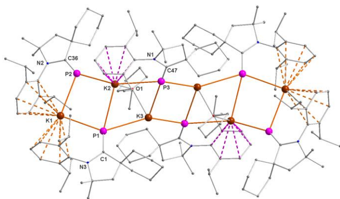
Figure 3. Molecular structure of complex 3 (depicted for atom connectivity only). H atoms and lattice THF molecules were omitted for clarity.
